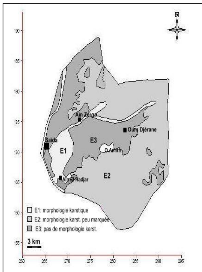
Figure 97: Couche Epikarst.
