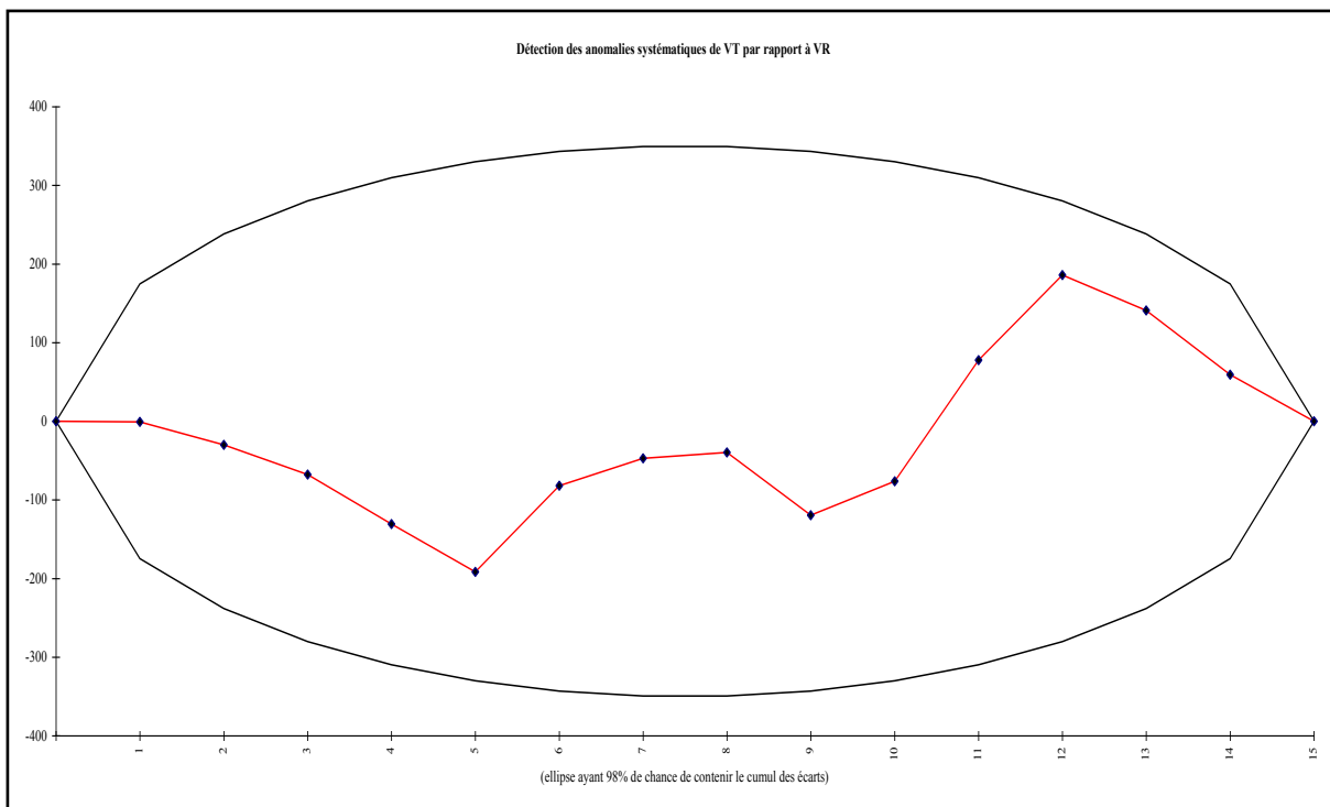
Figure 41: Ellipse de Bois - station -PK50.
