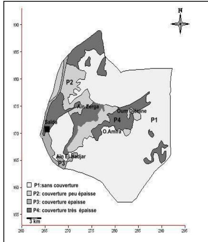
Figure 98: Couche Protection.
