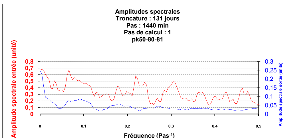
Figure 56: Amplitudes spectrales PK50 -cycle 1980-1981.
