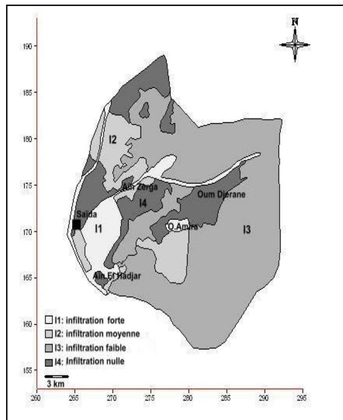
Figure 99: Couche Infiltration.
