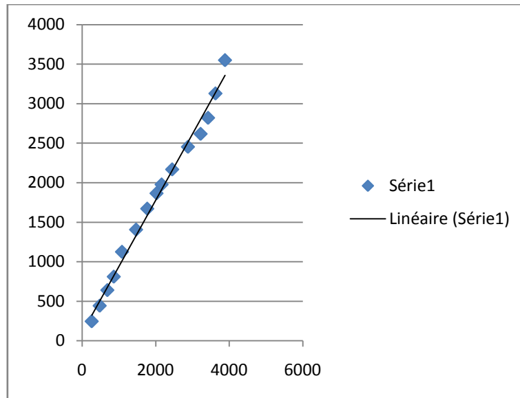
Figure 38: Double cumulé PK50-Sidi Boubekeur.
