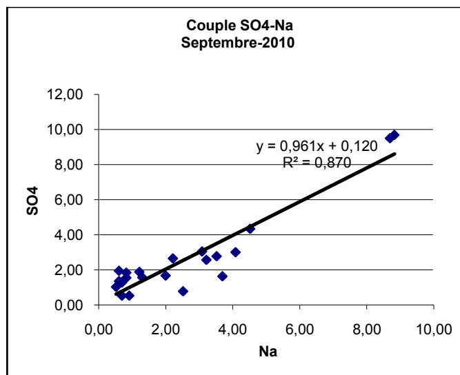
Figurexxx :Corrélation Na-SO4
