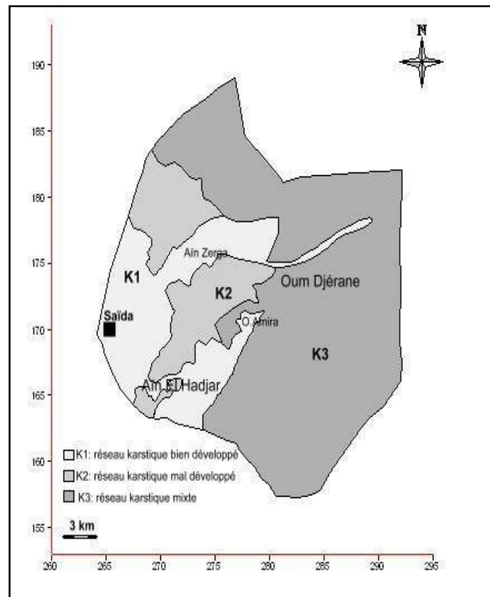
Figure 100: Couche Karst.
