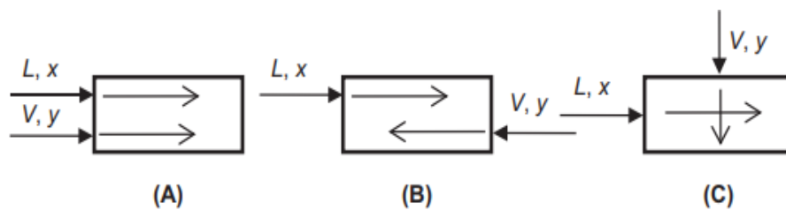
(A) A CO-courants. (B) A Contre-courants. (C) A Courants croisés.
